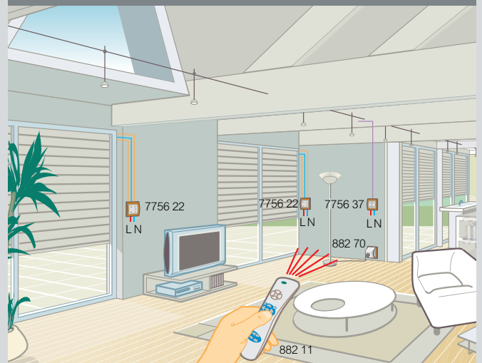
PLC/IR solution
